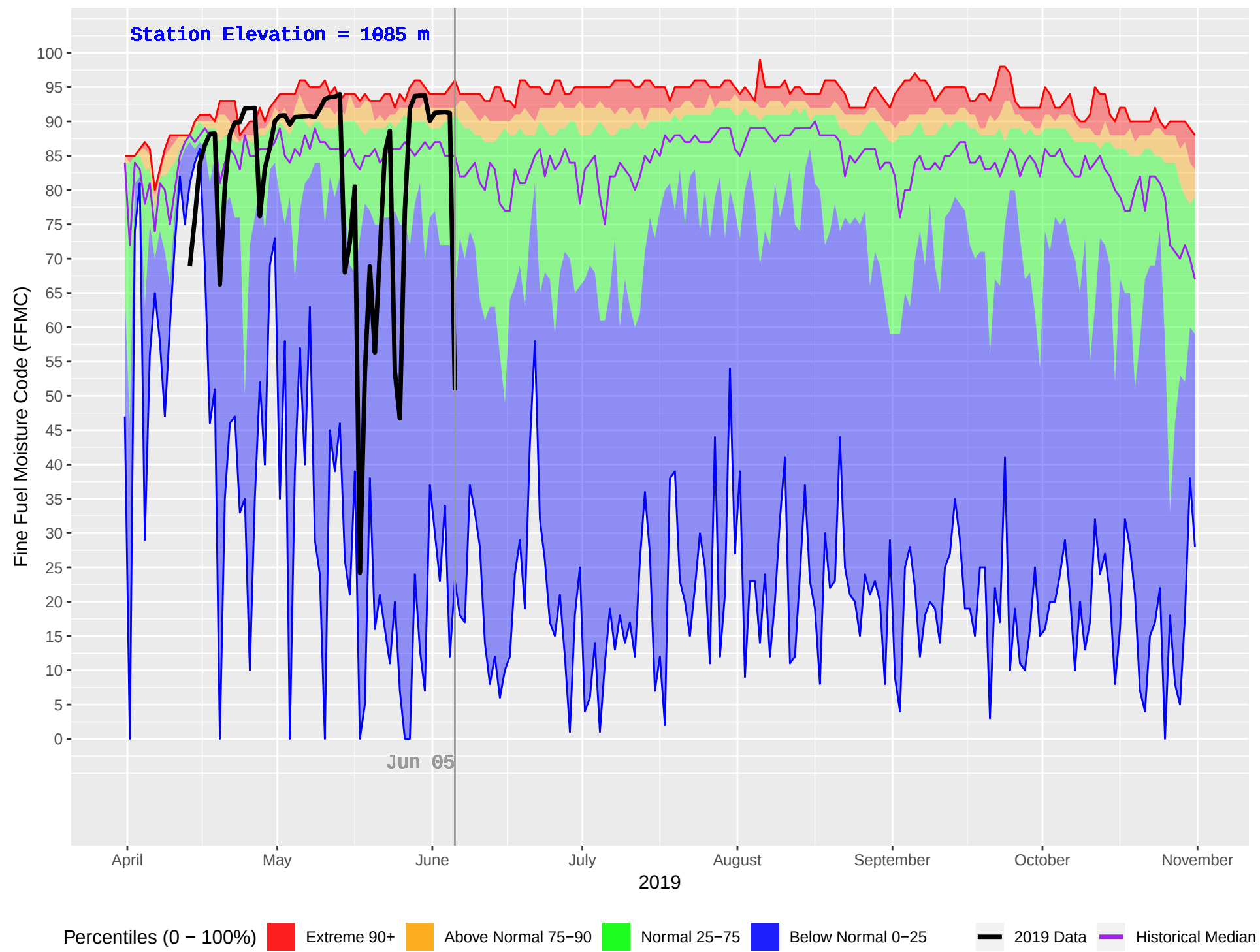
TAUTRI (206) : Historical (1970–2018) and Current (2019) Daily Fine Fuel Moisture Code (FFMC)
