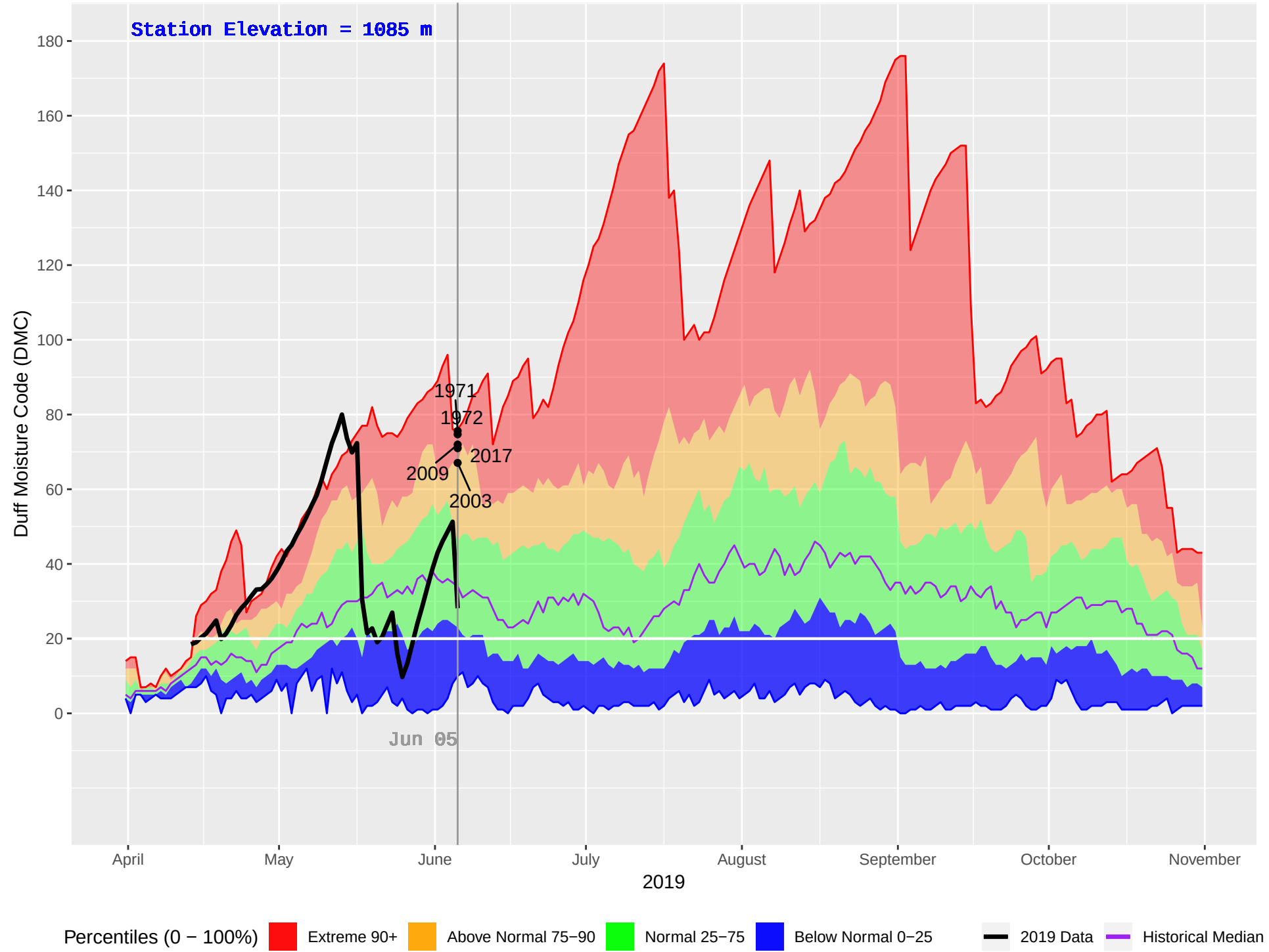
TAUTRI (206) : Historical (1970–2018), Current (2019) Daily Duff Moisture Code (DMC)
