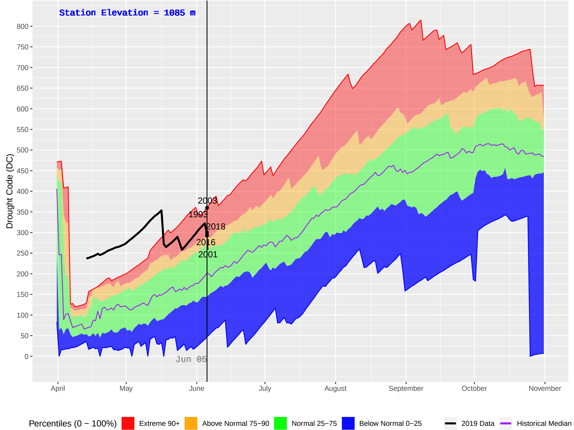
TAUTRI (206) : Historical (1970–2018) and Current (2019) Daily Drought Code (DC)
