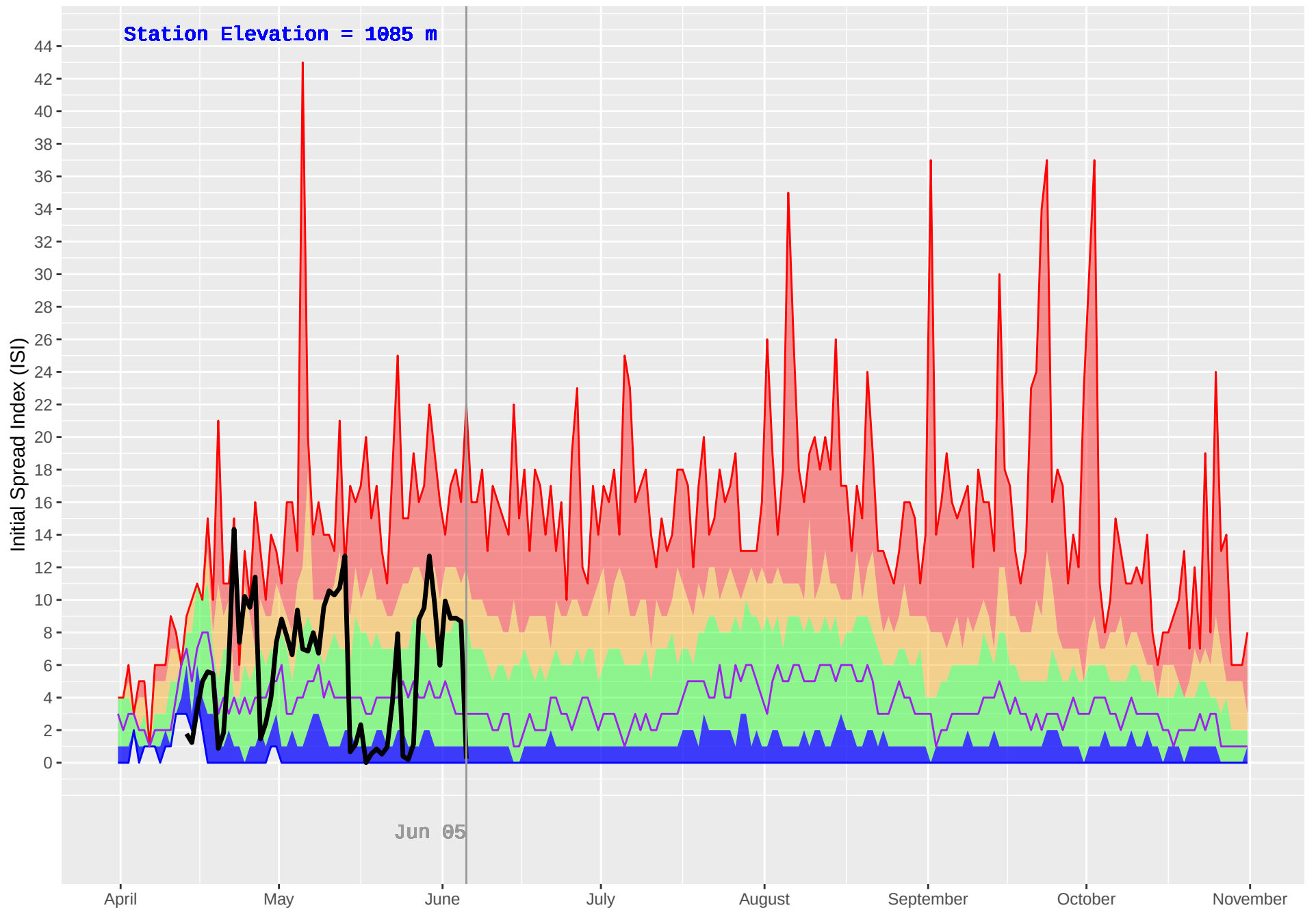
TAUTRI (206) : Historical (1970–2018) and Current (2019) Daily Initial Spread Index (ISI)
