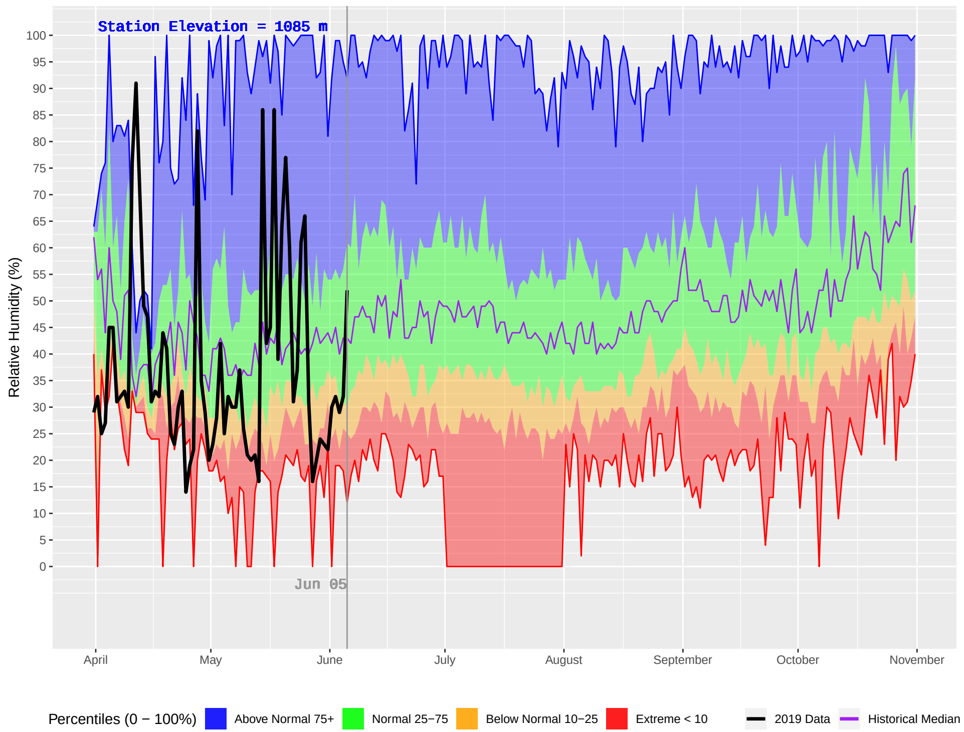
TAUTRI (206) : Historical (1970–2018) and Current (2019) Daily Relative Humidity
