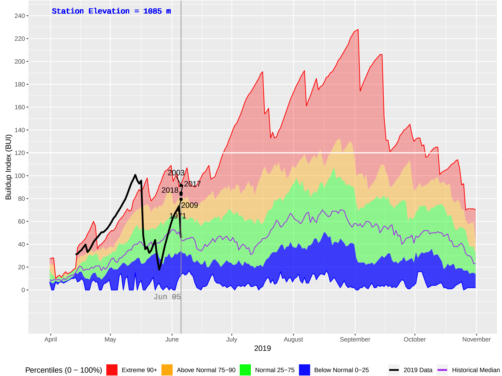
TAUTRI (206) : Historical (1970–2018), Current (2019) Daily Buildup Index (BUI)
