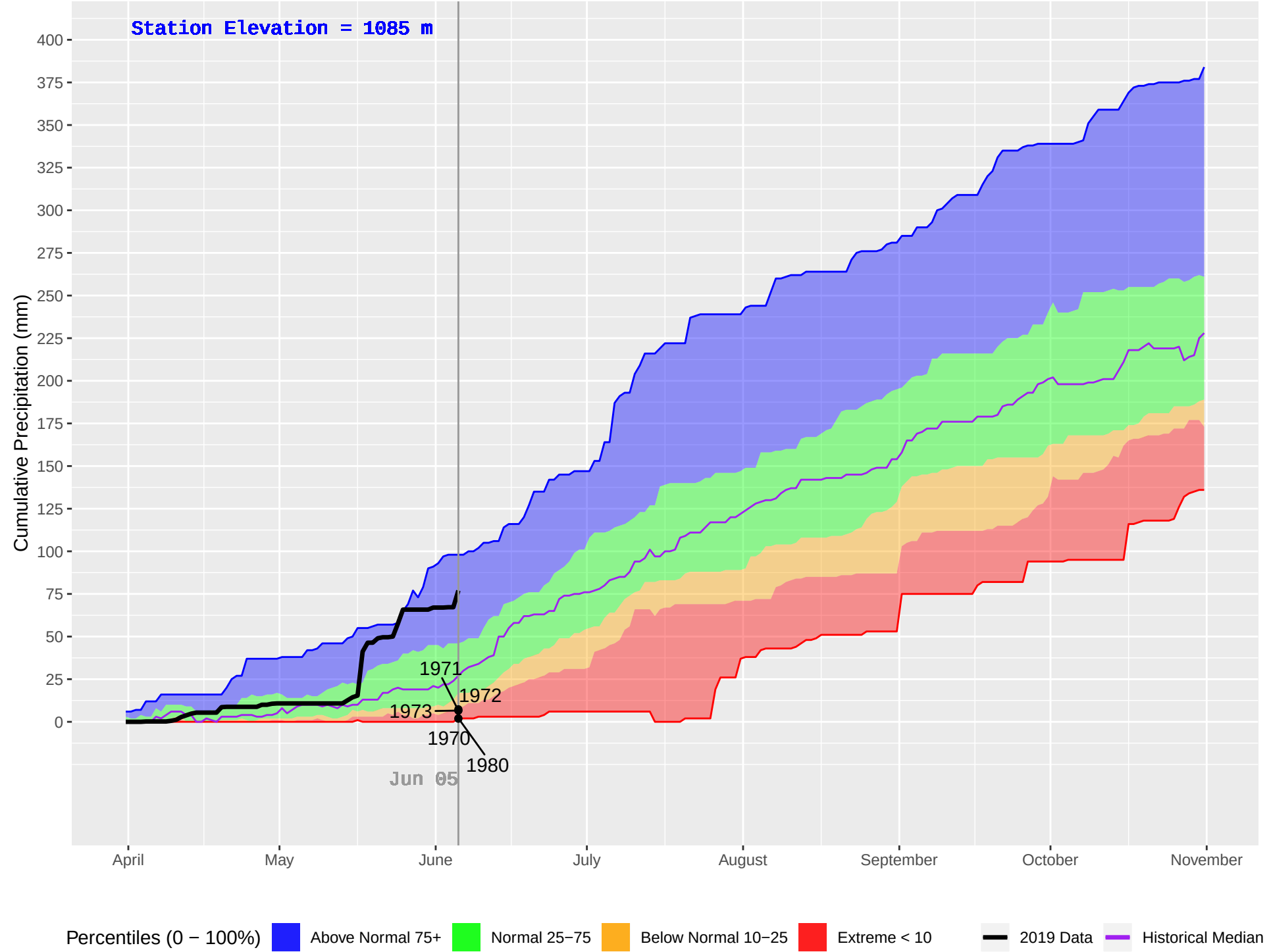
TAUTRI (206) : Historical (1970–2018), Current (2019) Daily Cumulative Precipitation
