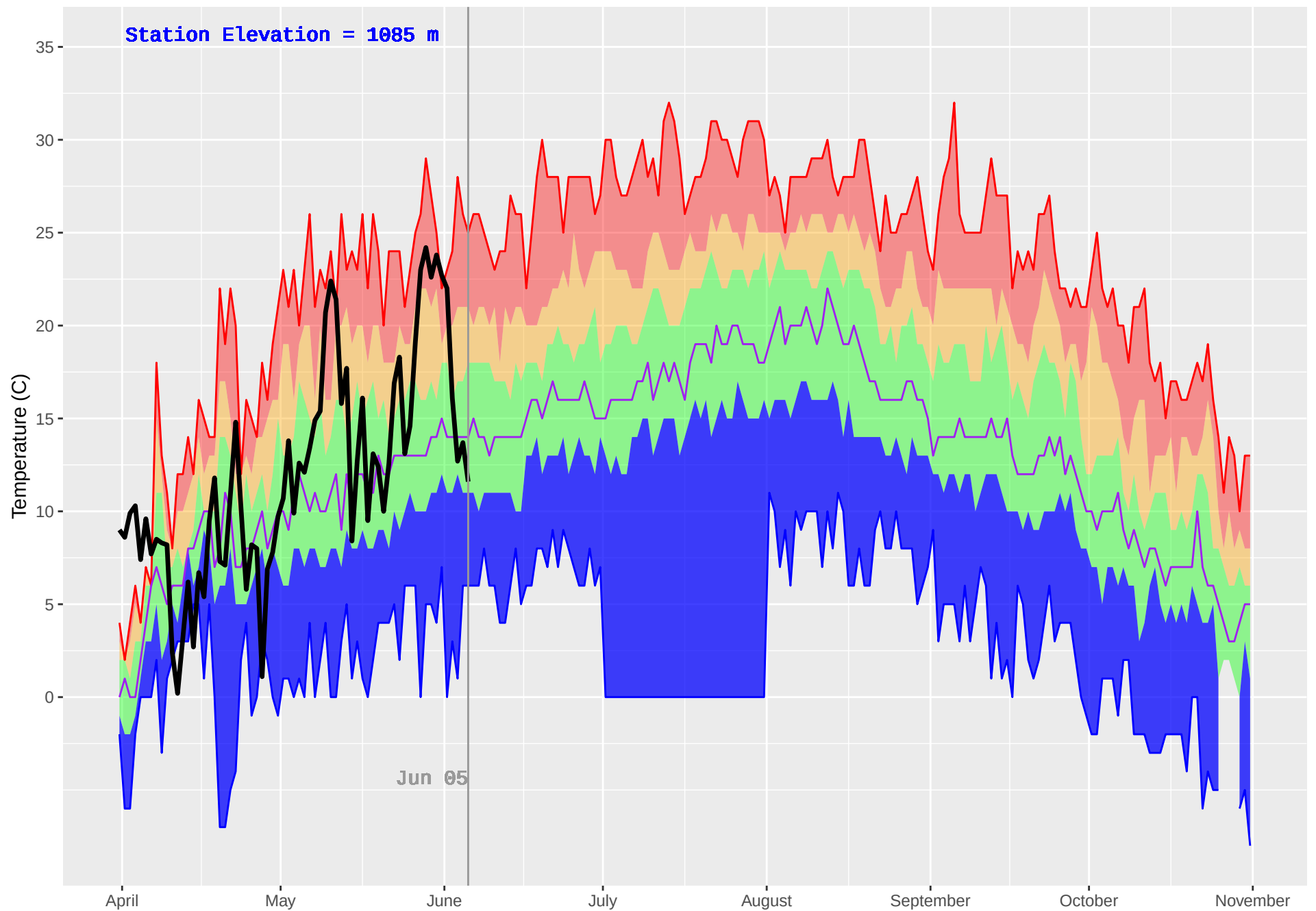
TAUTRI (206) : Historical (1970–2018) and Current (2019) Daily Temperature
