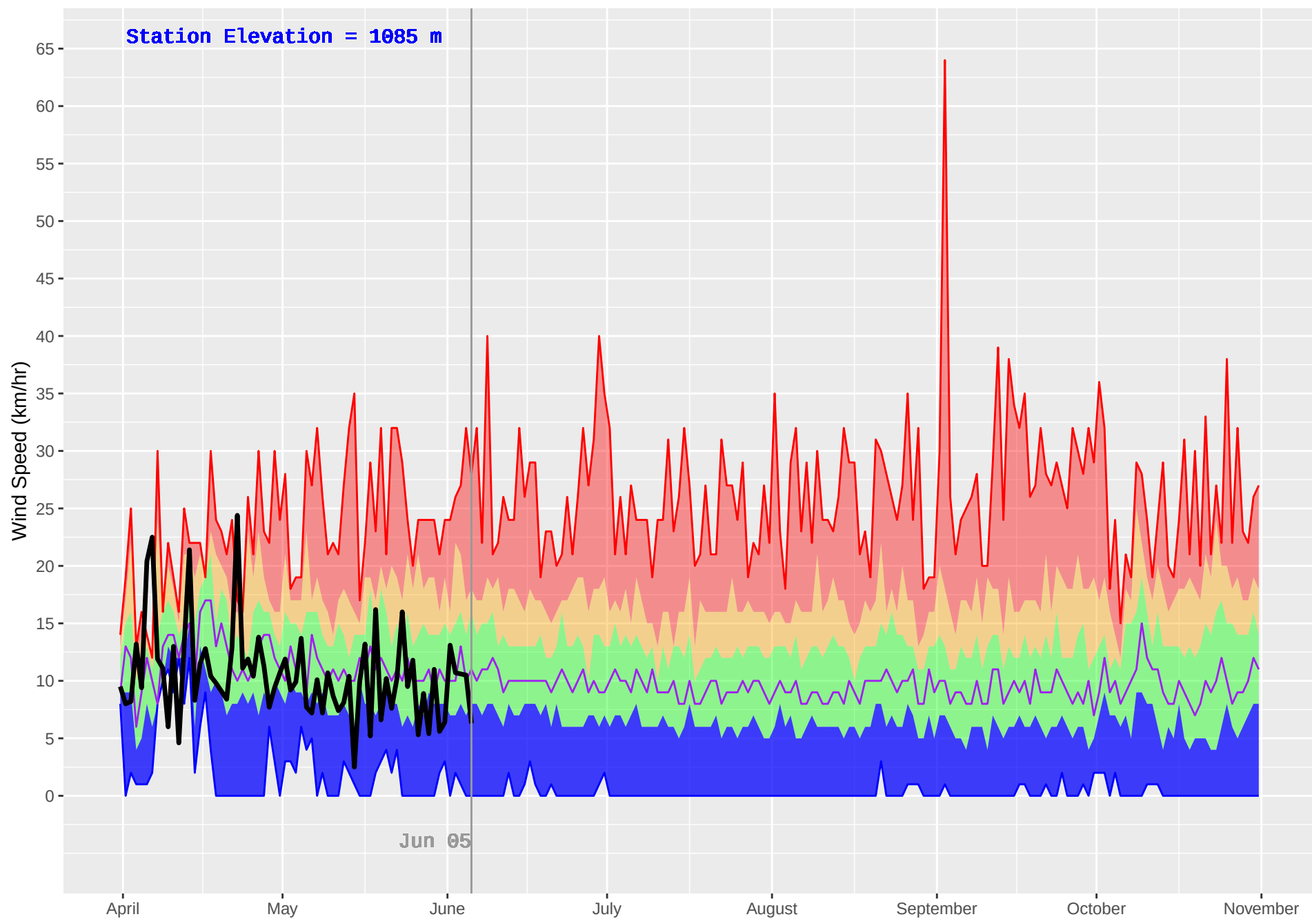
TAUTRI (206) : Historical (1970–2018) and Current (2019) Daily Wind Speed
